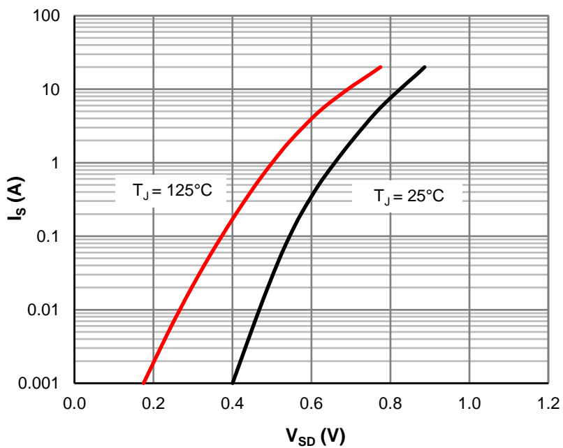
Figure 5: Body-Diode Characteristics
