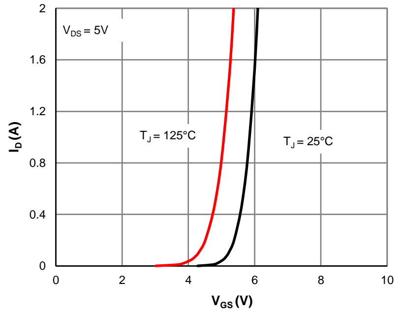
Figure 2: Transfer Characteristics
