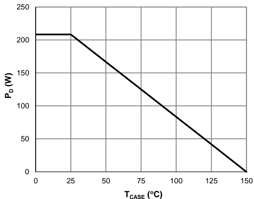
Figure 8: Power De-rating
