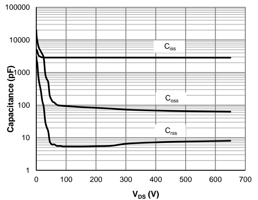
Figure 6: Capacitance Characteristics
